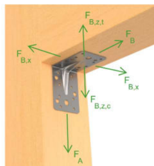
PILLAR
