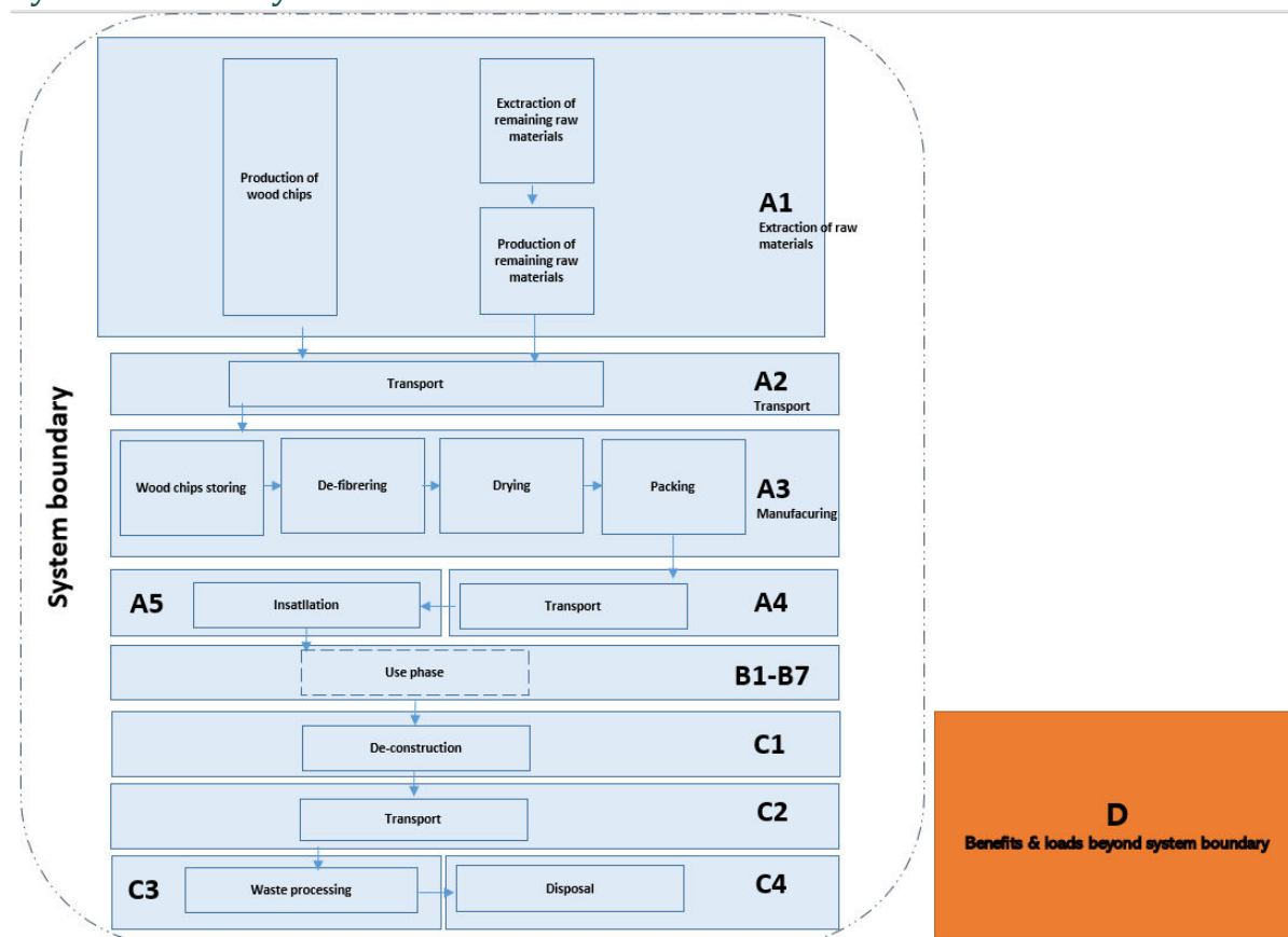
Figure 2. System boundaries.
